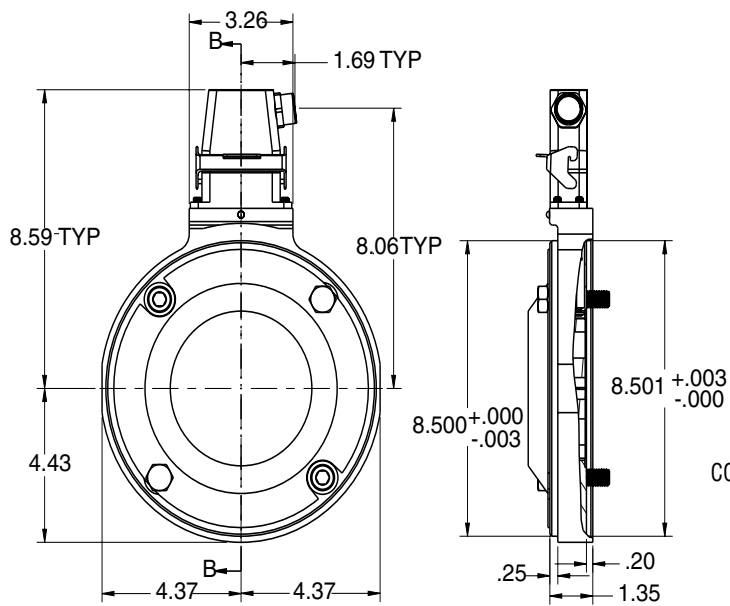
SECTION B-B PIE PAN COVER OPTION
