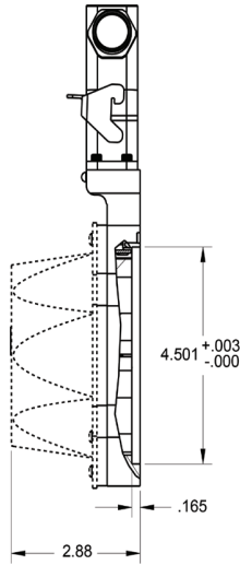
SECTION A-A PLASTIC COVER OPTION
