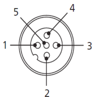
Male 5-pin M12 (Code A)
