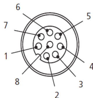
Male 8-pin M12 (Code A)
