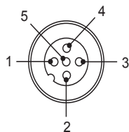
Male 5-pin M12 (Code A)
