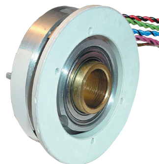
Servo ring mounting with integral flexure is size 10 pancake resolver equivalent
