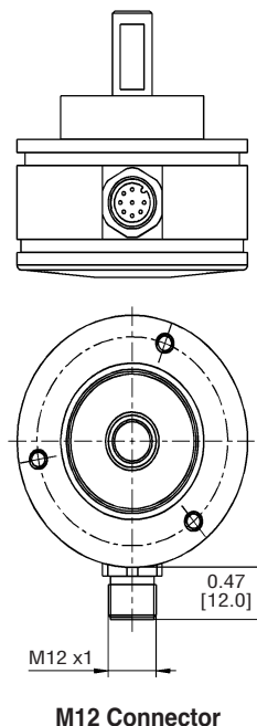
M12 Connector
